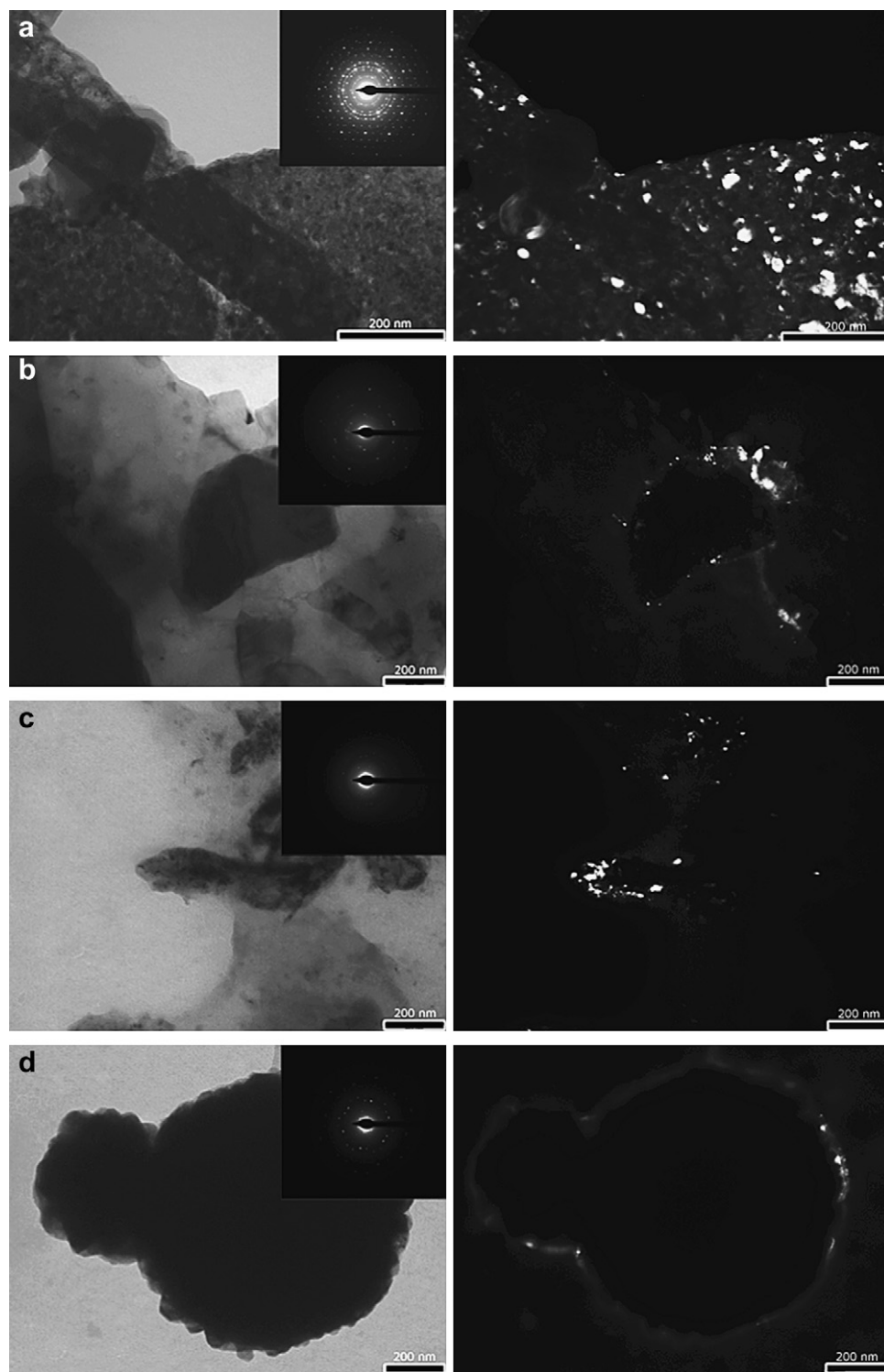
Figure 2 Bright-field and corresponding dark-field TEM images of nanoparticles and aggregates observed in Zincum met : (a) 30c (SBL), (b) 200c (SBL), (c) 30c (WSI), (d) 200c (WSI). Inset – SAED patterns of the corresponding nanoparticle/aggregate.
